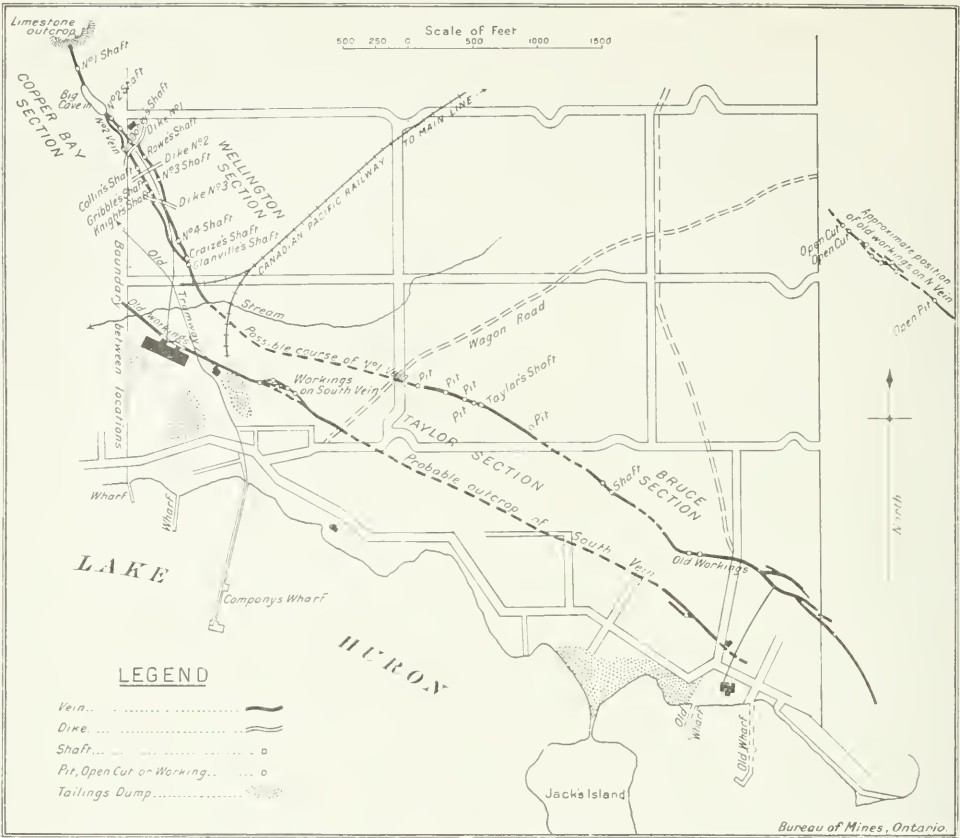
Plan showing copper veins and workings at Bruce Mines, on the north shore of Lake Huron.
